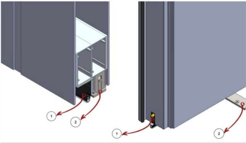
2, top and bottom pivot system
